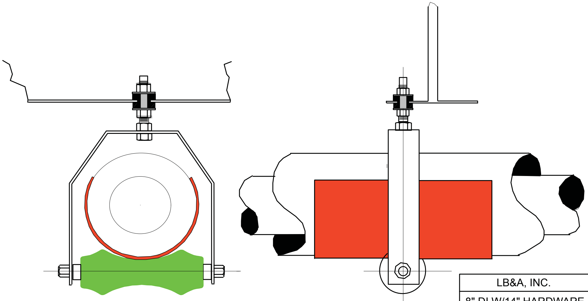
CLEVIS HANGER W/ INSULATING BUSHING
