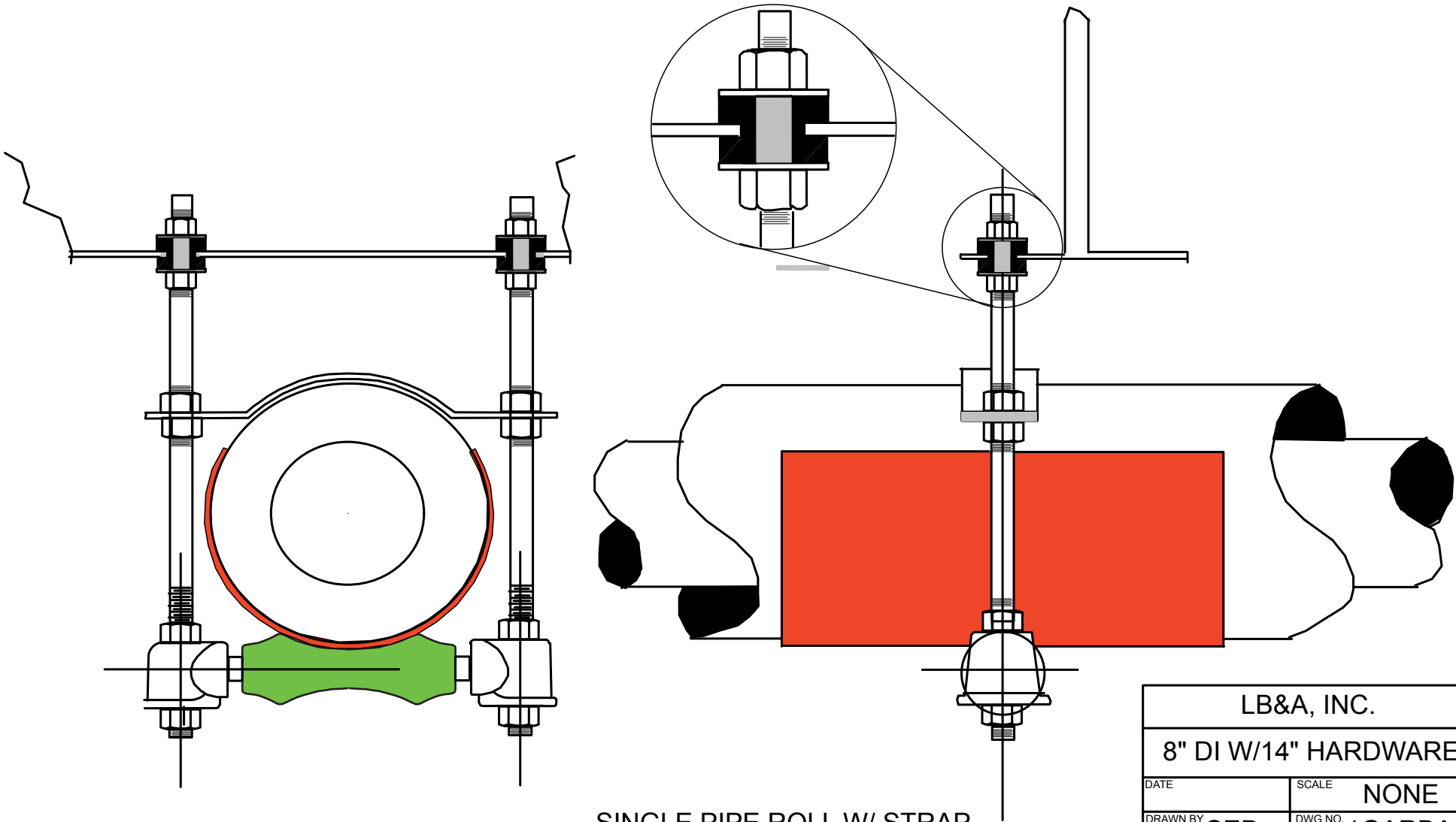
SINGLE PIPE ROLL W/ STRAP W/ INSULATING BUSHINGS
